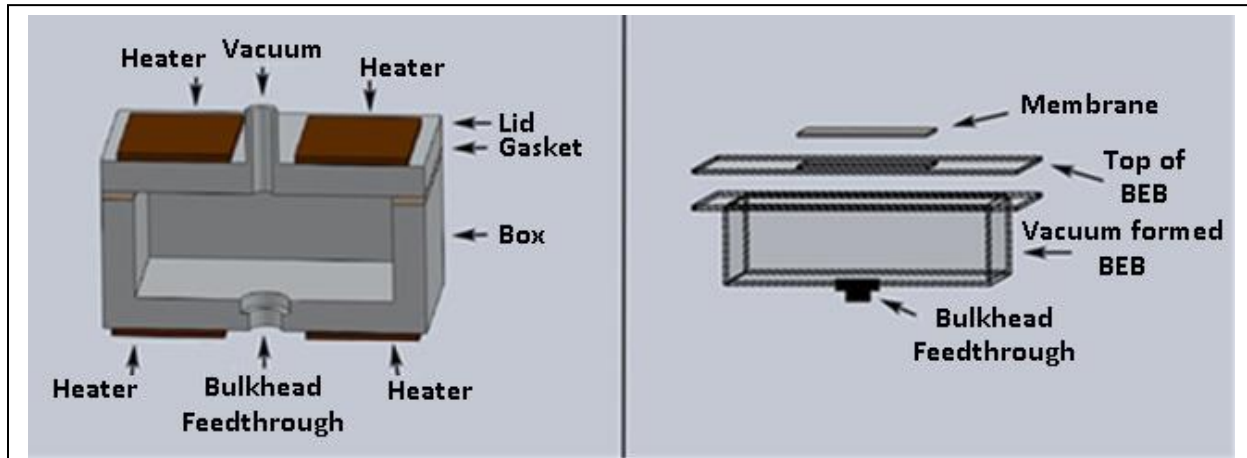
Figure 1. The BEB evaporator (left) and BEB (right).
