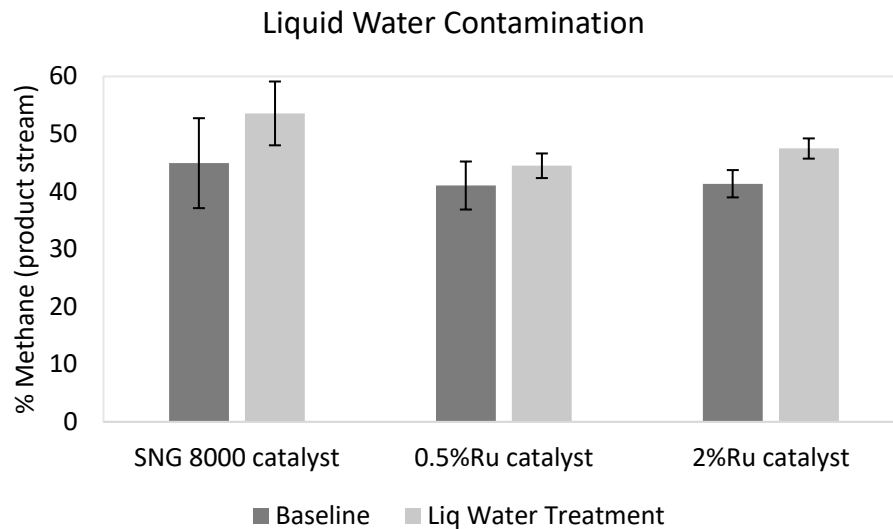
Figure 7: CH 4 production before and after liquid water exposure for a) SNG 8000 catalyst, b) 0.5% Ru catalyst and c) 2.0% Ru catalyst
