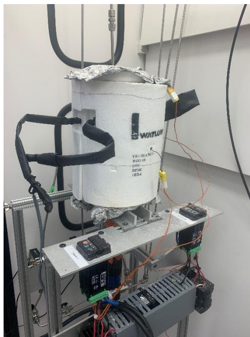
Figure 3: Sabatier assembly used during testing
