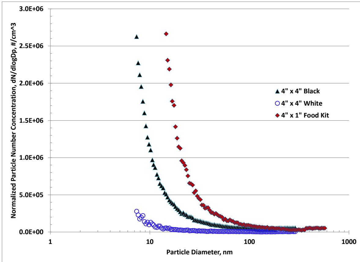
Figure 3: SMPS particle size distribution measured while mating/demating Velcro in a purged glovebox. The highest concentrations are from flight qualified Velcro vs. the white sample, which was purchased at a retail store.
