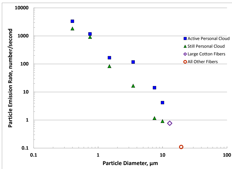
Figure 1: Personal cloud and fiber emission rates combined to account for a larger size range of lint data. Solid symbols are from personal cloud data (You et al.) and open symbols are the original fiber emission data in Table 1.
