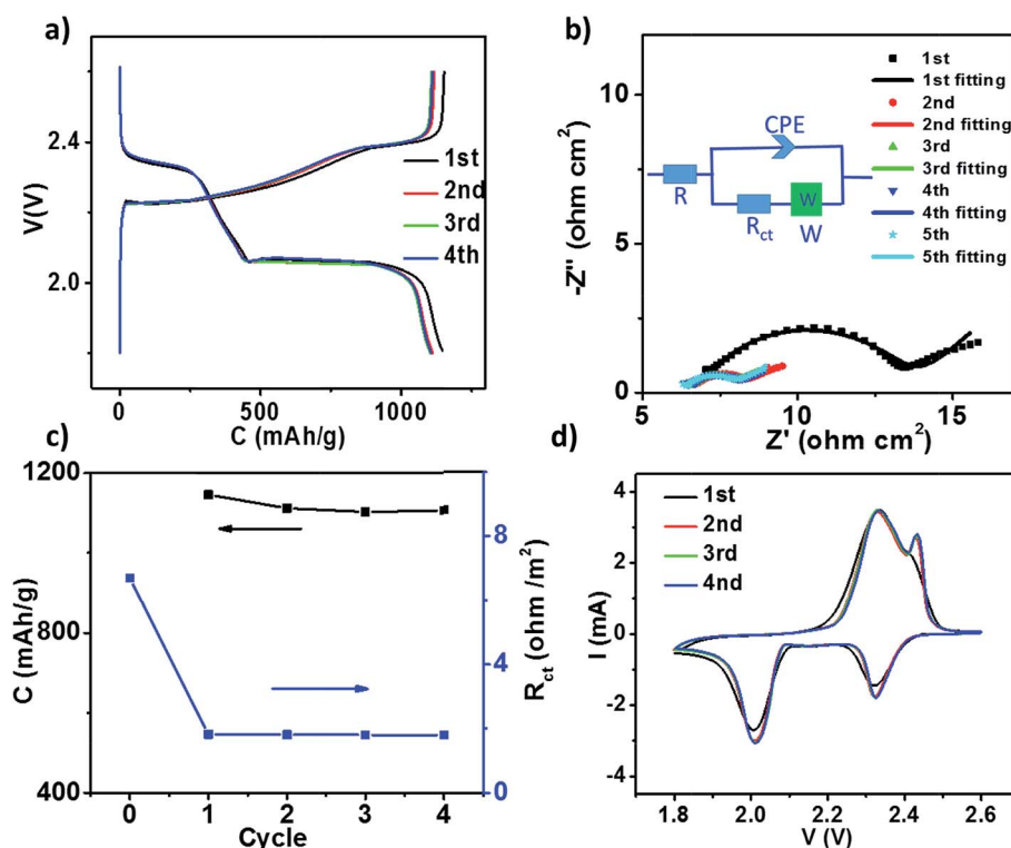
Fig. 2 (a) The behavior of the first few cycles at 0.2C of a cell, and (b) the Nyquist plot of the same cell from the EIS measurement before discharge and after each discharge–charge cycle at 2.6 \text{ V} ; (c) specific capacity and charge transfer resistant evolution in the first few cycles. (d) CV behavior for a typical cell in the first few CV cycles measured at 0.1 \text{ mV s}^{-1} .
