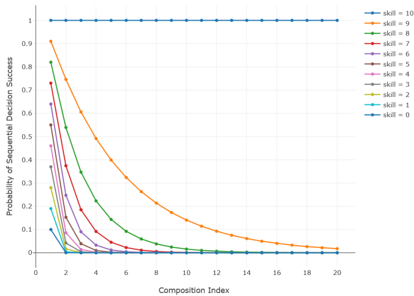
Figure 3. Probability of sequential decision success.
