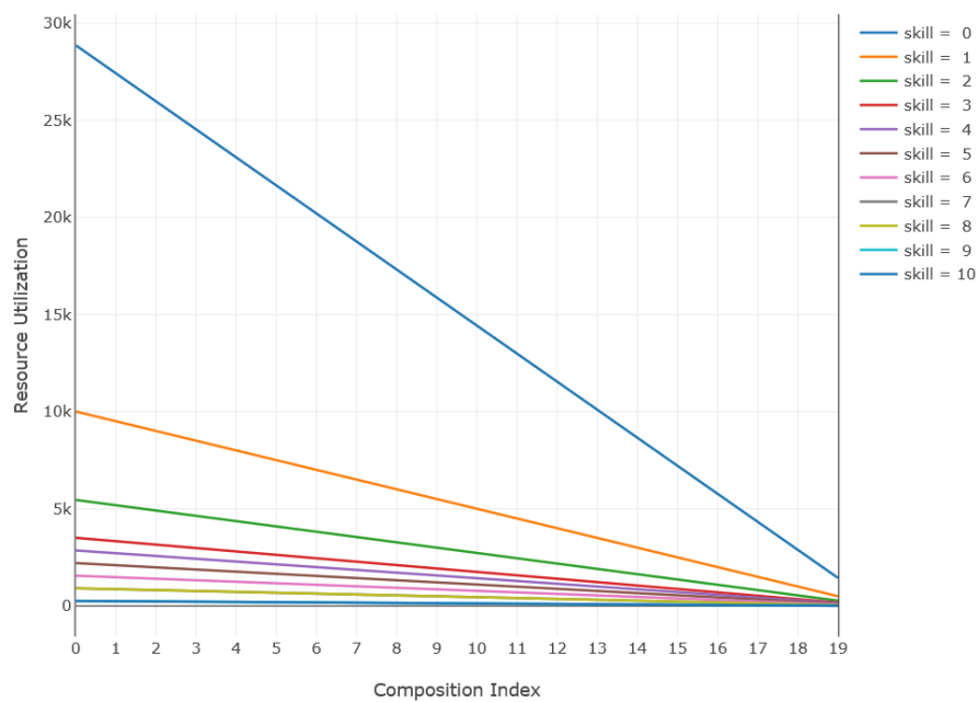
Figure 5. Cumulative resource utilization.
