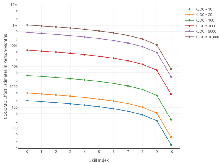
Figure 7. Constructive Cost Model (COCOMO) effort estimation for various program sizes measured in thousands of lines of source code (KLOC).
