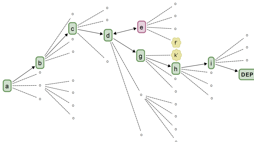
Figure 2. A simple development space (DSpace) excerpt with highlighted development paths (DPaths).
