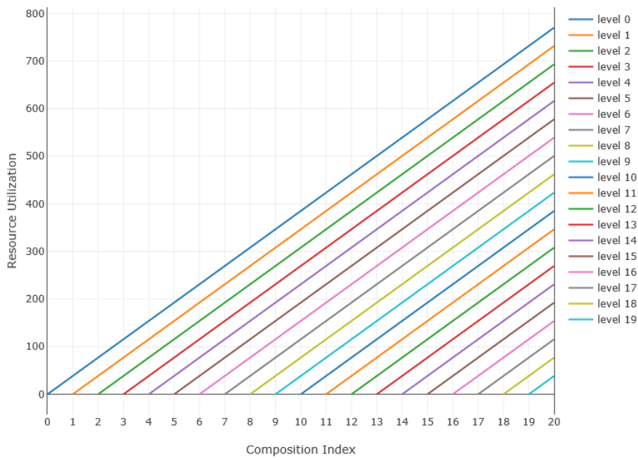
Figure 4. Cumulative resource utilization as estimated from each composition index (l).
