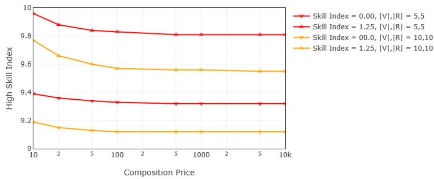
Figure 6. Skill Indices for 16:1 estimate ratios by price.
