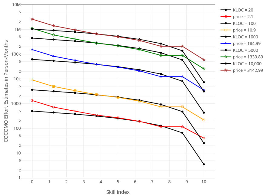
Figure 8. Statistical Agent-based Model of Development and Evaluation (SAbMDE)-to-COCOMO effort estimation comparison for various KLOC values.
