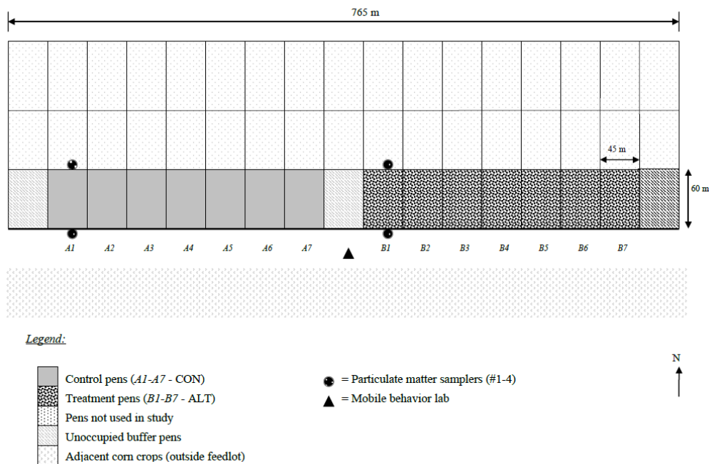
Figure 1. Schematic of experimental setup for particulate matter ( PM_{2.5} ) and behavior sampling. A total of 4 PM_{2.5} samplers were used to measure PM_{2.5} concentrations upwind (south side) and downwind (north side) in the south and southwest pens of the feedlot, in 1 pen per treatment per day. The 4 PM_{2.5} samplers were moved daily from 1 of the 7 pens (per treatment) to the next. For example, on d 1, upwind and downwind locations were sampled in pens A1 and B1 as shown above. On day 2, upwind and downwind locations were sampled for PM_{2.5} in pens A2 and B2 etc. Behavioral measures were recorded in 15 min scan sampling mode by live observation using a camera that was mounted to a 10-m high rotating tripod on top of a mobile behavior lab from 1600 and 2100 on the same days when PM_{2.5} was measured. The mobile behavior lab remained at the depicted location throughout the duration of the study. Prevailing wind direction was from the South.
