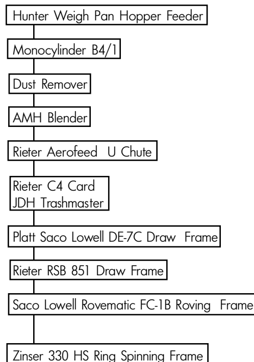
Figure 1: Processing Flow
