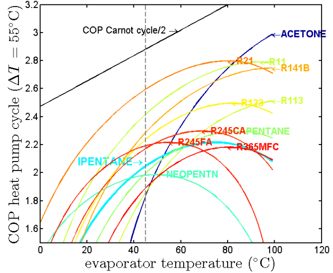
Figure 5 Figure of Merit for a heat pump
