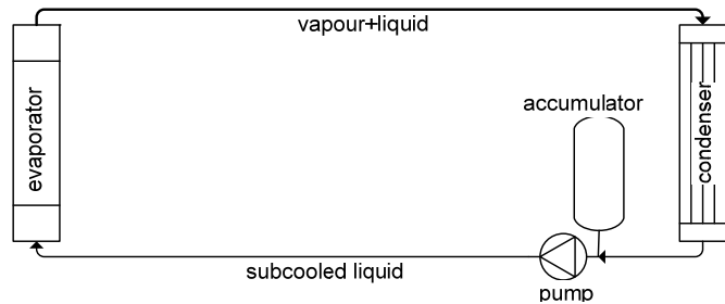
Figure 2 Schematic drawing of a two-phase pumped loop
