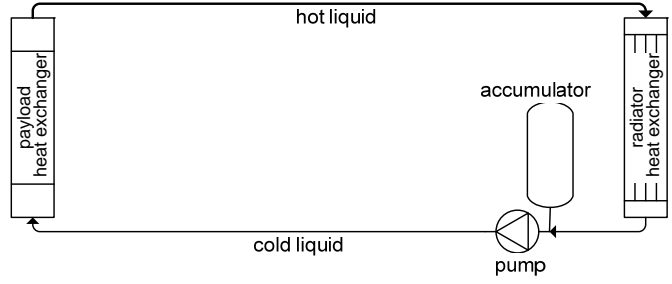
Figure 7 Schematic drawing of a single-phase pumped loop
