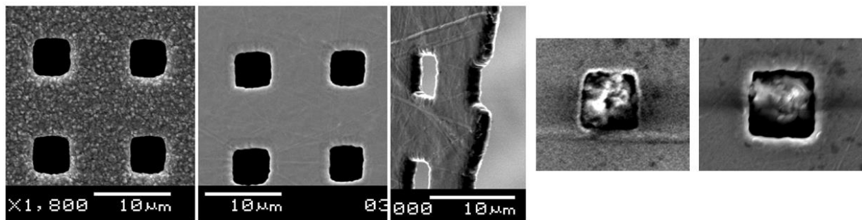
Figure 1. Scanning electron microscope images of plasmonic Ni mesh. The mesh is produced by Precision Eforming ( www.precisioneforming.com ) and has a lattice parameter of 12.7 \mu\text{m} , a square hole width of \sim 5 \mu\text{m} , and a thickness of \sim 2 \mu\text{m} . When air is pumped through the mesh, dust particles of a specific size are trapped in the mesh holes as shown on the right-hand side. Scatter-free IR absorption spectra can be recorded of individual particles trapped in this manner because IR light runs along the metal surface rather than going directly through the holes.
