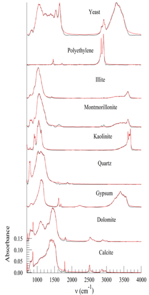
Figure 3. Average IR spectra of calibrant particles. Spectra of individual calibrant particles were averaged and fit to the permittivity defined by a damped harmonic oscillator model.
