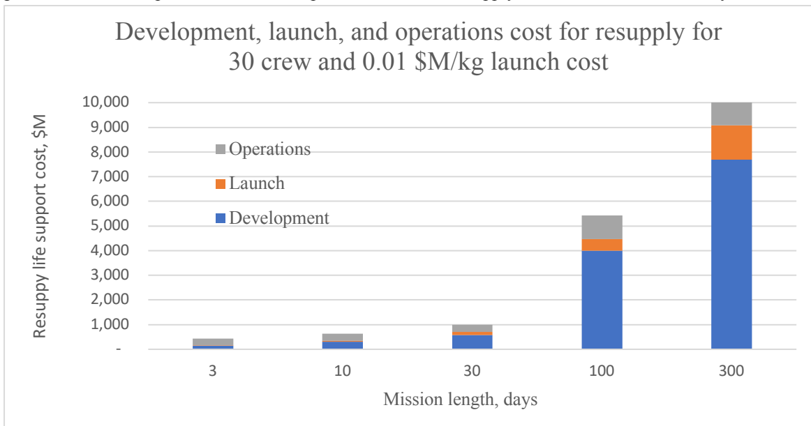
Figure 4. Cost breakdown for resupply for 30 crew and 0.01 $M/Kg launch cost
