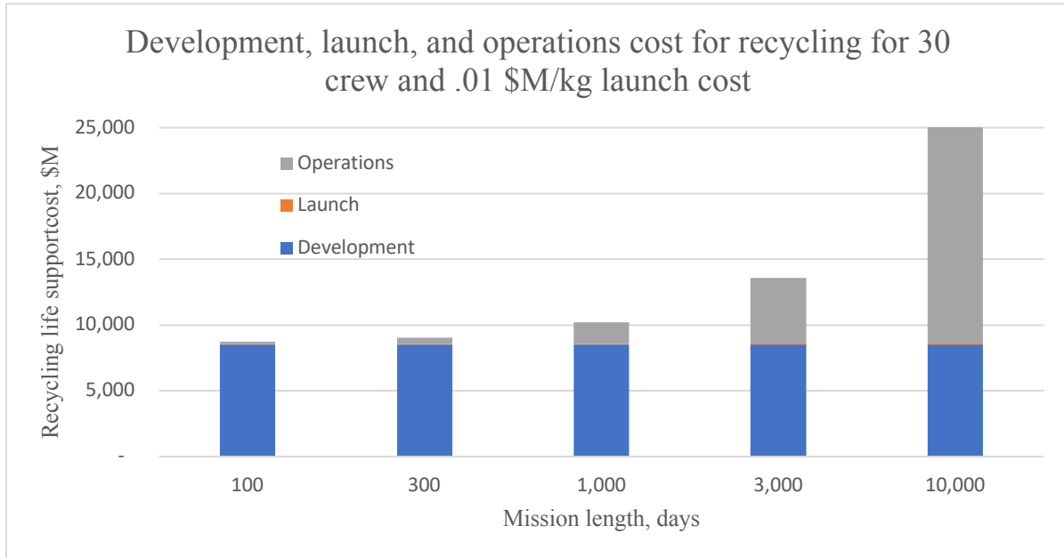
Figure 5. Cost breakdown for recycling for 30 crew and 0.01 $M/Kg launch cost
