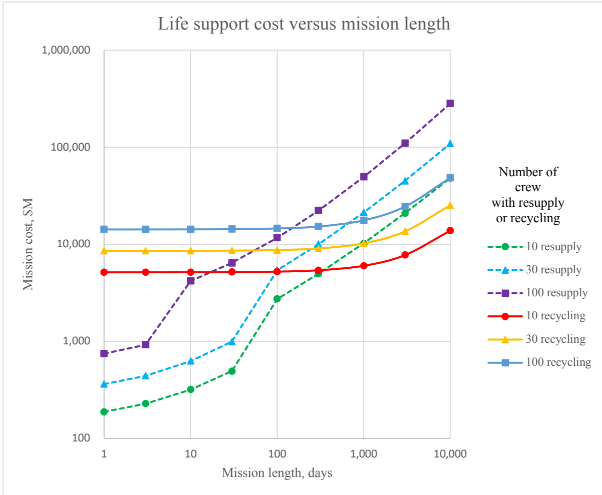
Figure 3. Life support cost versus mission length for a launch cost of 0.01 $M/kg ($10 k/kg).
